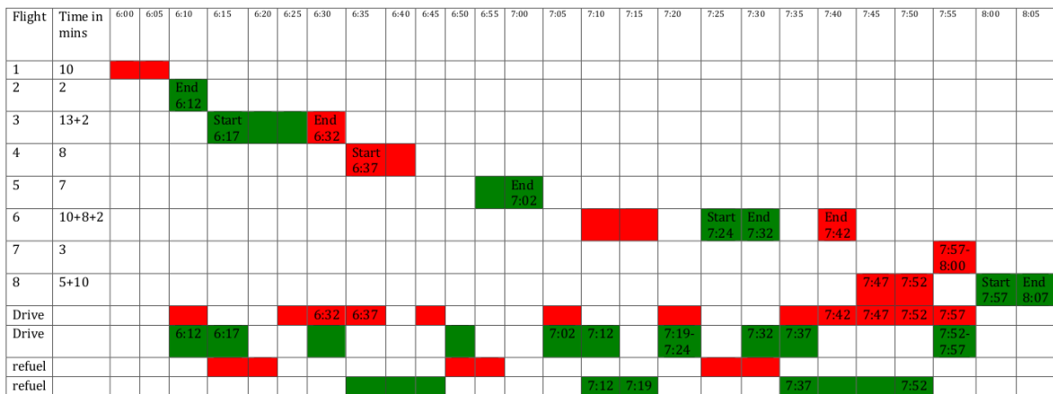
Figure 2: The gantt chart shows when which truck serves which flight. In some cases both trucks are needed for a single aircraft. Black times indicate start and end times.
