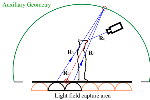
Figure 9: The depth correction process. The incident illumination images we need to sample for the spatial interpolation are, as before, determined by the intersection of the backwards-traced ray \vec{R}_0' with the incident light field plane. Instead of just using the direction of \vec{R}_0 as the lookup for the directional interpolation, depth correction recalculates the directions such that they converge at the intersection of \vec{R}_0 with the auxiliary geometry.
