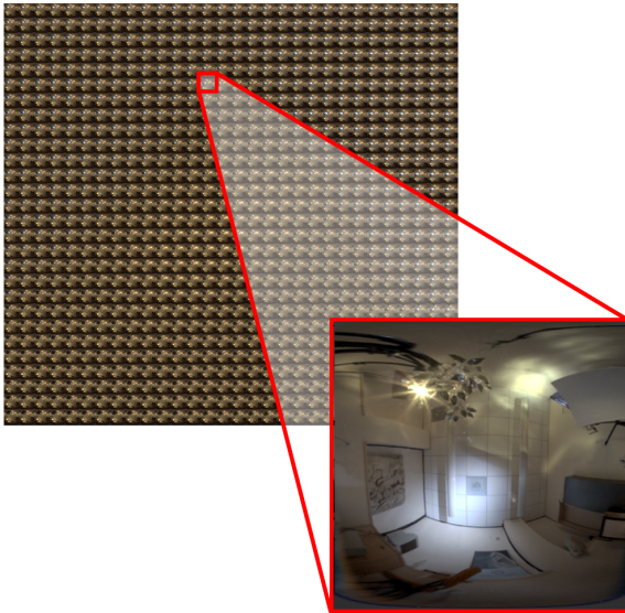
Figure 7: High fidelity incident light field data. A 30 × 30 spatial resolution and 400 × 400 directional resolution incident light field captured by the high fidelity device.
