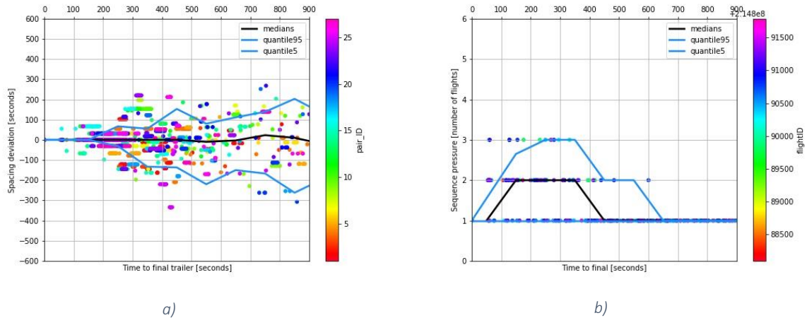
Figure 37 – January 29th, 6:00 – 7:00, (total 28 aircraft) - a) Spacing deviation- min = -334s, max = 268s, avg = 3.02, std = 71.89, 90 th quantile width = 465, b) Sequence pressure- window size = 120s, min = 1, max = 3, avg = 1.34, std = 0.57
