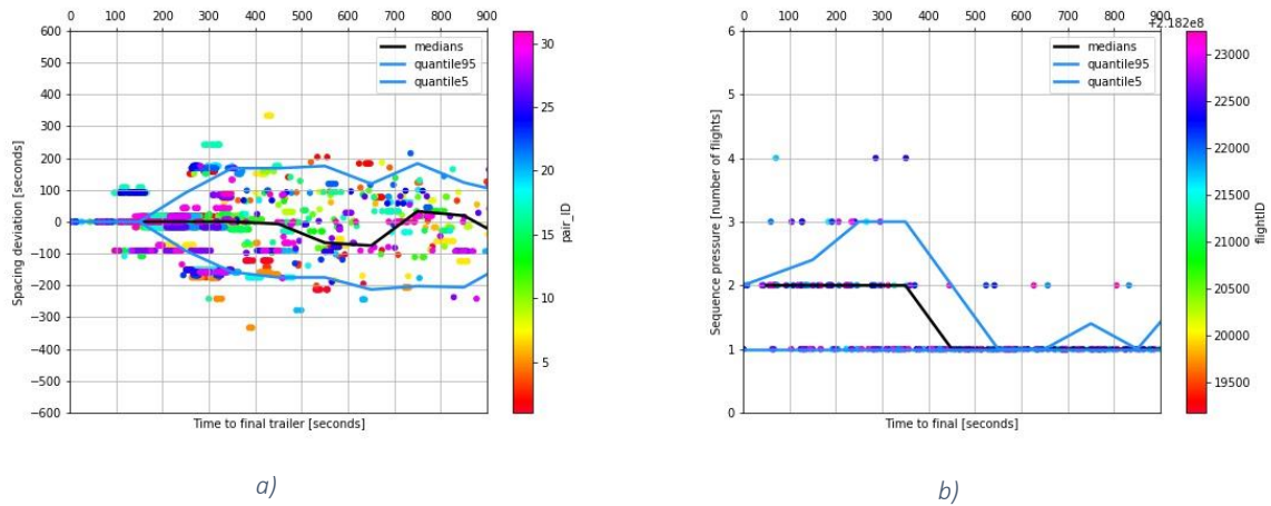
Figure 14 – May 16 th , 5:00 – 6:00, (total 32 aircraft) - a) Spacing deviation, \min = -333s , \max = 333s , \text{avg} = 9.82 , \text{std} = 85.6 , 90^{\text{th}} quantile width = 385.35, b) Sequence pressure, window size = 90s, \min = 1 , \max = 4 , \text{avg} = 1.34 , \text{std} = 0.6
