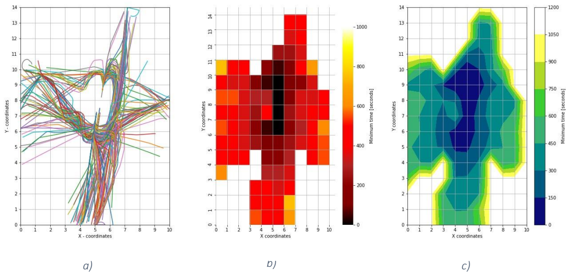
Figure 38 – January 29 th , 6:00 – 0:00, (total 271 aircraft), min = 0s, max = 743s, avg = 358s, std = 167s - a) Flight trajectories, b) Heatmap, c) Contour plot
