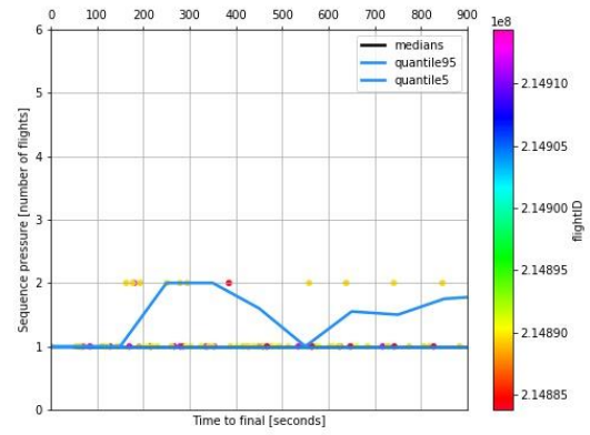
Figure 42 – January 29th, 0:00 – 6:00, (total 11 aircraft - a) Spacing deviation- min = -225s, max = 132s, avg = 7.39, std = 78.02, 90 th quantile width = 301.75, b) Sequence pressure- window size = 120s, min = 1, max = 2, avg = 1.13, std = 0.34
