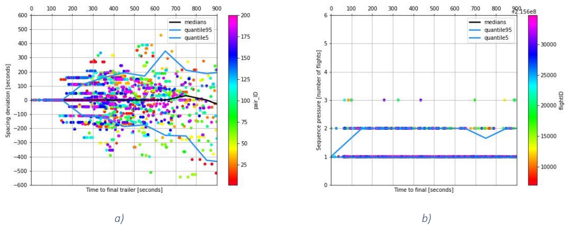
Figure 31 – February 26th, 6:00 – 0:00, (total 201 aircraft) - a) Spacing deviation, min = -544s, max = 458s, avg = 1.21, std = 109.89, 90 th quantile width = 612.05, b) Sequence pressure, window size = 120s, min = 1, max = 3, avg = 1.13, std = 0.36
