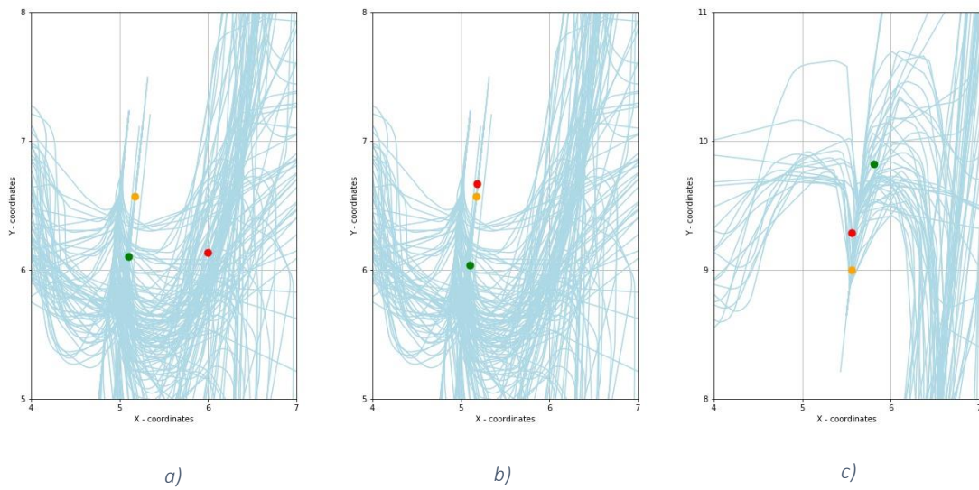
Figure 40 – January 29 th , 6:00 – 0:00, (total 271 aircraft) – a) Sequence pressure for 214891029 (time 7:02:18), b) Sequence pressure for 214891029 (time 7:21:45). c) Sequence pressure for 214895732 (time 9:32:46)
