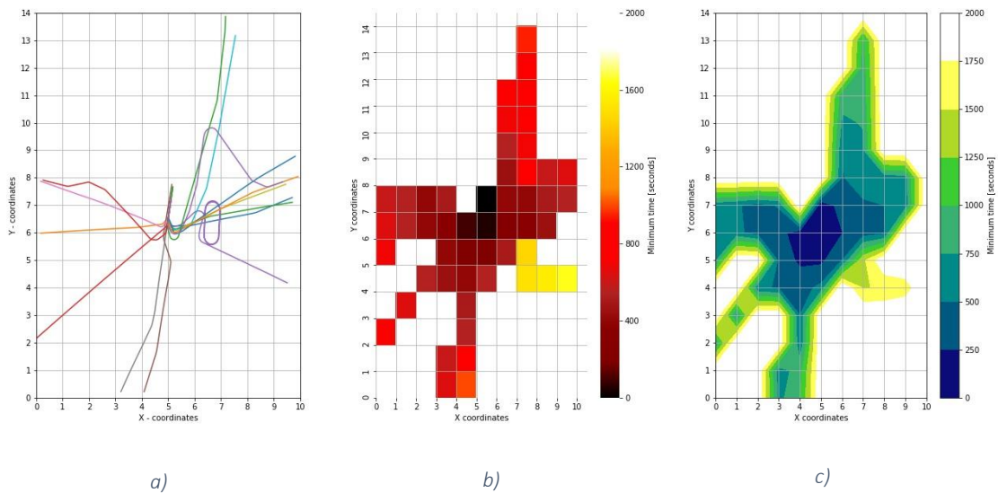
Figure 32 - February 26th, 00:00 – 06:00, (total 15 aircraft) - min = 0s, max = 1636s, avg = 615s, std = 342s - a) Flight trajectories, b) Heatmap, c) Contour plot
