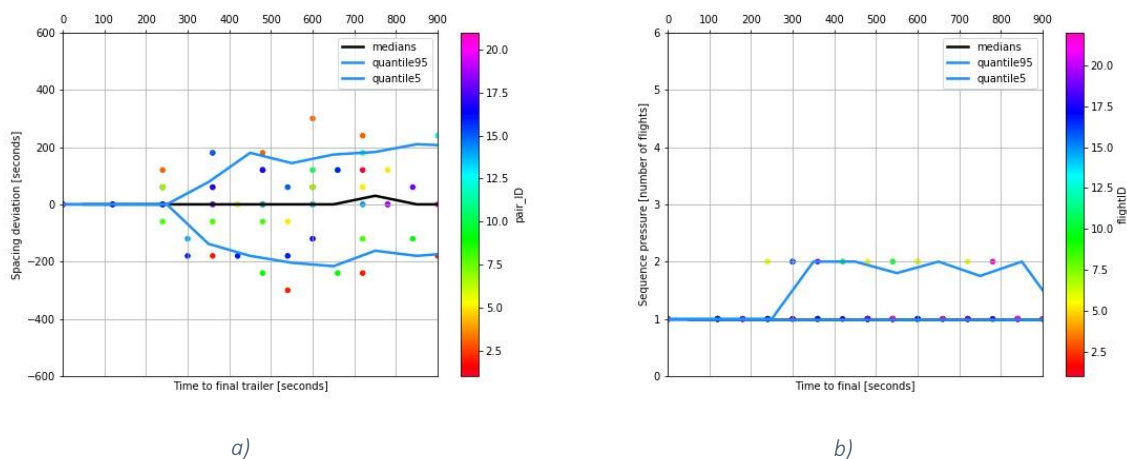
Figure 44 - Simulated optimized routes (22 aircraft) – a) Spacing deviation, min = -300s, max = 300s, avg = 6.74s, std = 109.46s, 90 th quantile width = 390, b) Sequence pressure, window size = 120s, min = 1, max = 2, avg = 1.05, std = 0.21
