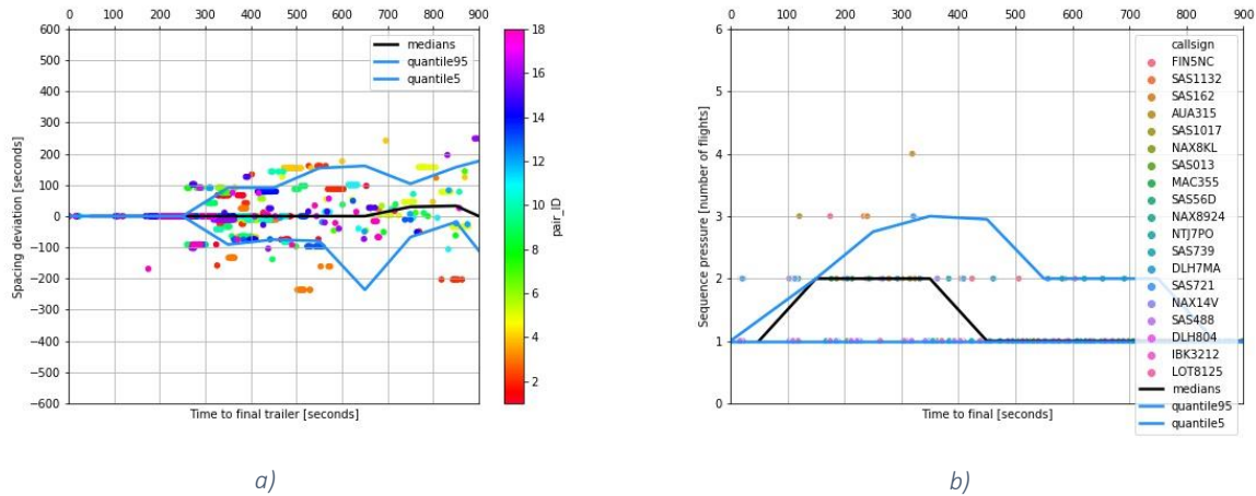
Figure 46 - 3 rd of October 2017 (total of 19 aircraft) – a) Spacing deviation, min = -236s, max = 249s, avg = 6.74s, std = 64.72s, 90 th quantile width = 390, b) Sequence pressure, window size = 120s, min = 1, max = 4, avg = 1.33, std = 0.55
