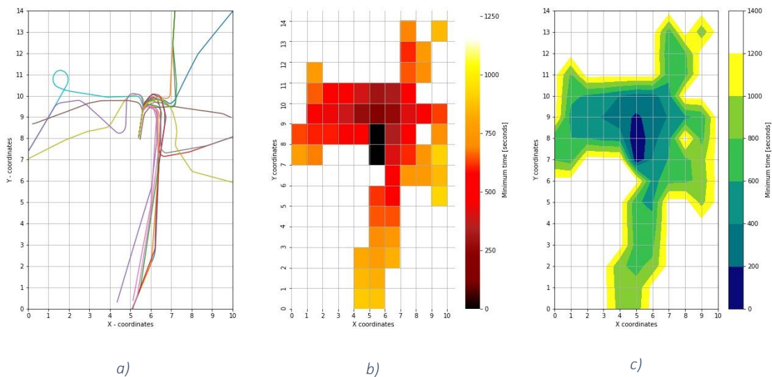
Figure 45 – 3 rd of October 2017 (total of 19 aircraft), min = 0s, max = 1273s, avg = 998s, std = 360s, a) Flight trajectories, b) Heatmap, c) Contour plot
