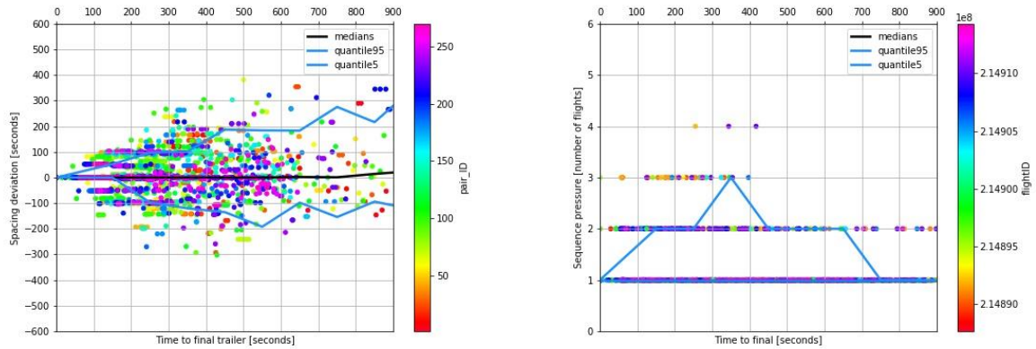
Figure 39 – January 29th, 6:00 – 0:00, (total 271 aircraft) - a) Spacing deviation- min = -302s, max = 382s, avg = 5.67, std = 74.51, 90 th quantile width = 429.55, b) Sequence pressure, window size = 120s, min = 1, max = 4, avg = 1.19, std = 0.44
