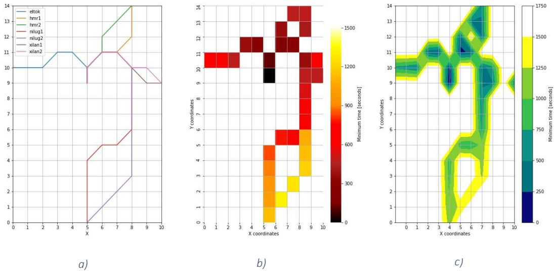
Figure 43 – Simulated optimized routes (22 aircraft), min = 0s, max = 1320s, avg = 644s, std = 341s - a) Flight trajectories, b) Heatmap, c) Contour plot
