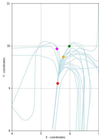
Figure 47 – Outlier investigation, aircraft positions
