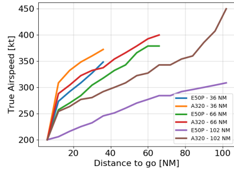
Figure 1. Speed profiles inside the TMA for an E50P and an A320.
